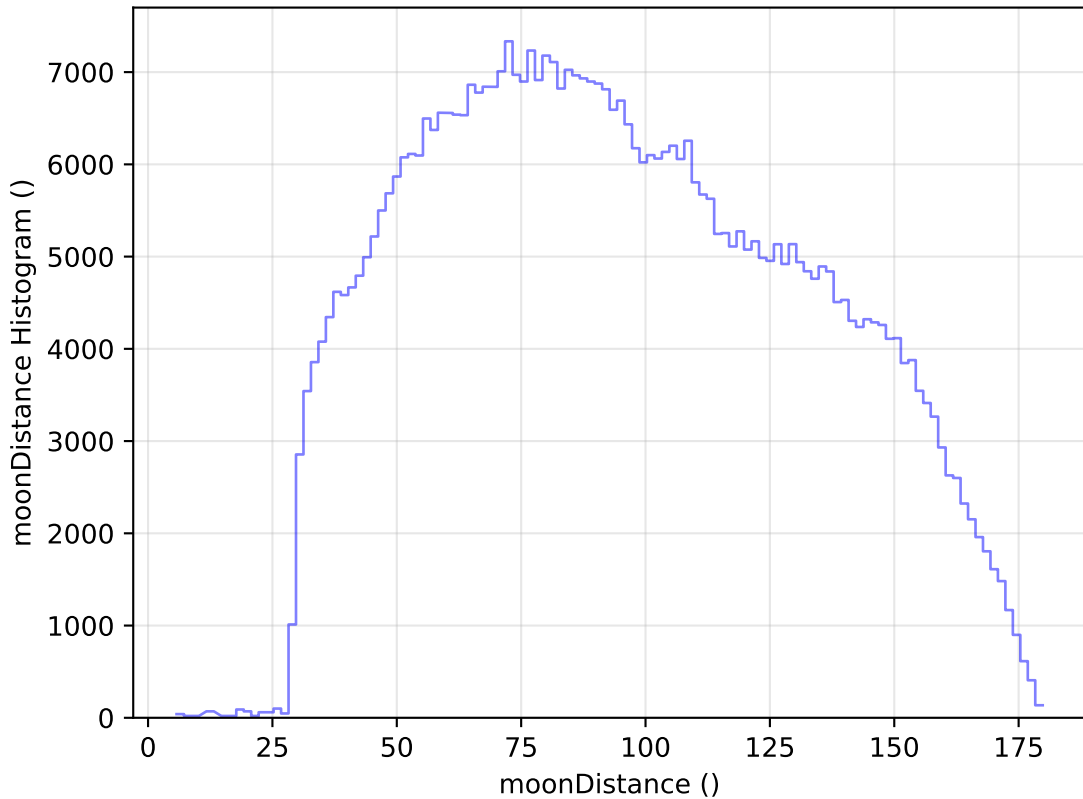
too_elab_r32_d2_gz_v3.4_10yrs WFD i band: moonDistance Histogram
