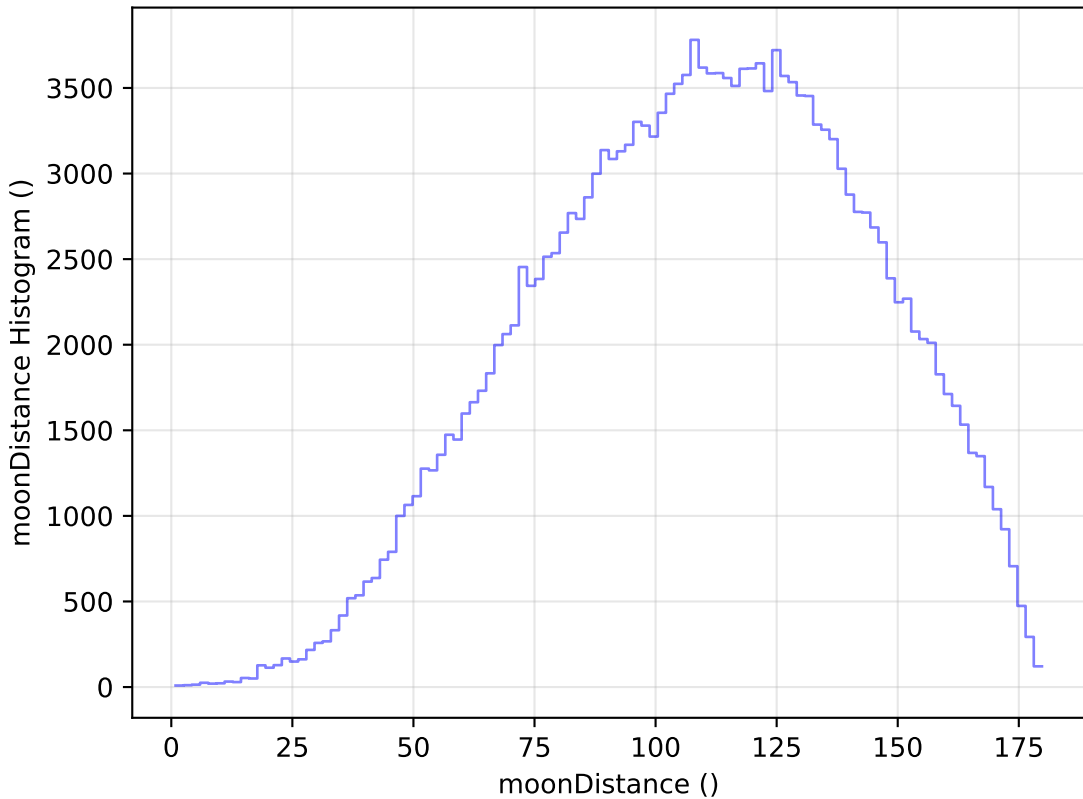
too_elab_r32_d2_gz_v3.4_10yrs WFD g band: moonDistance Histogram
