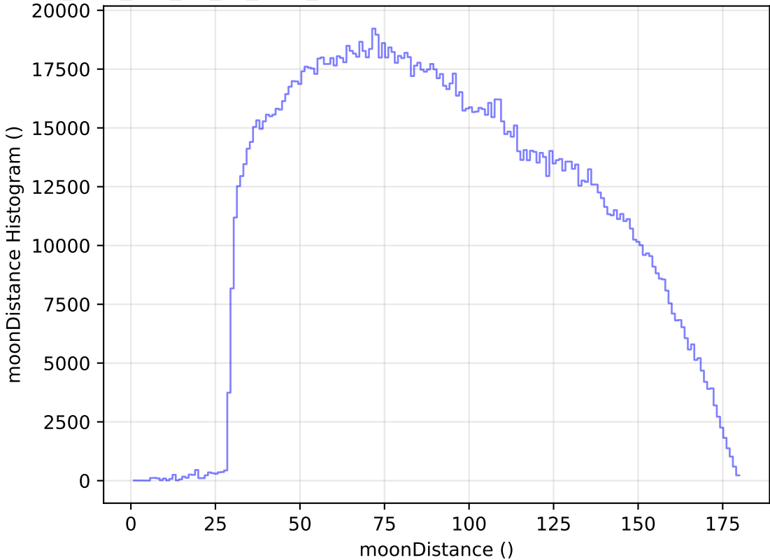
too_elab_r32_d2_gz_v3.4_10yrs WFD all bands: moonDistance Histogram
