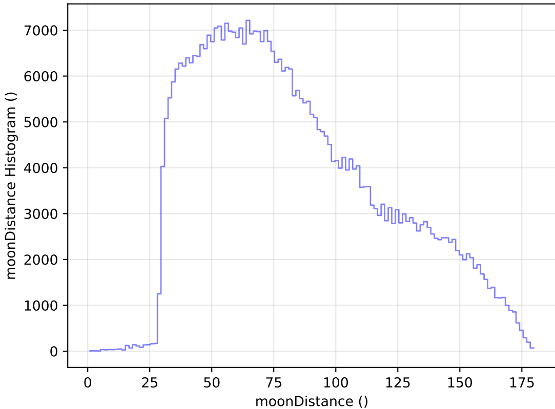
too_elab_r32_d2_gz_v3.4_10yrs All sky z band: moonDistance Histogram
