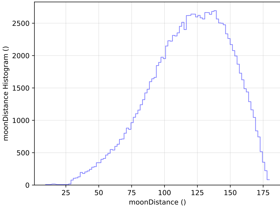
too_elab_r32_d2_gz_v3.4_10yrs All sky u band: moonDistance Histogram
