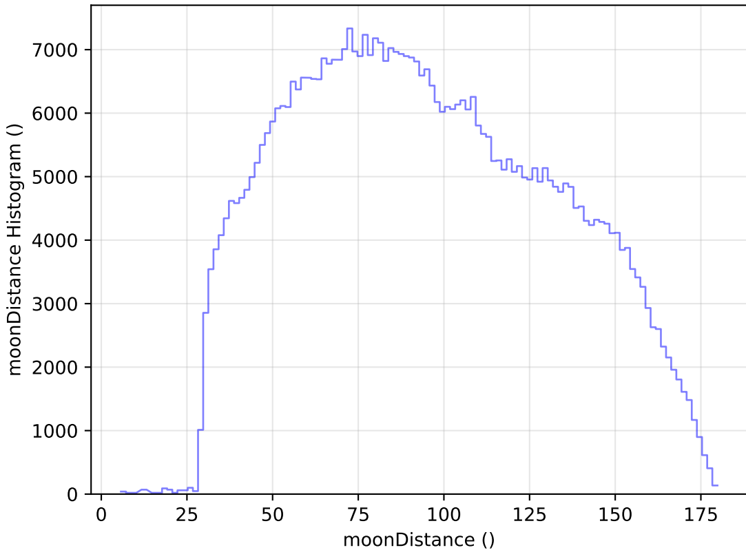
too_elab_r32_d2_gz_v3.4_10yrs All sky i band: moonDistance Histogram
