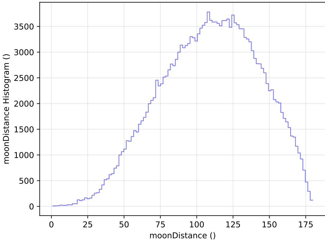
too_elab_r32_d2_gz_v3.4_10yrs All sky g band: moonDistance Histogram
