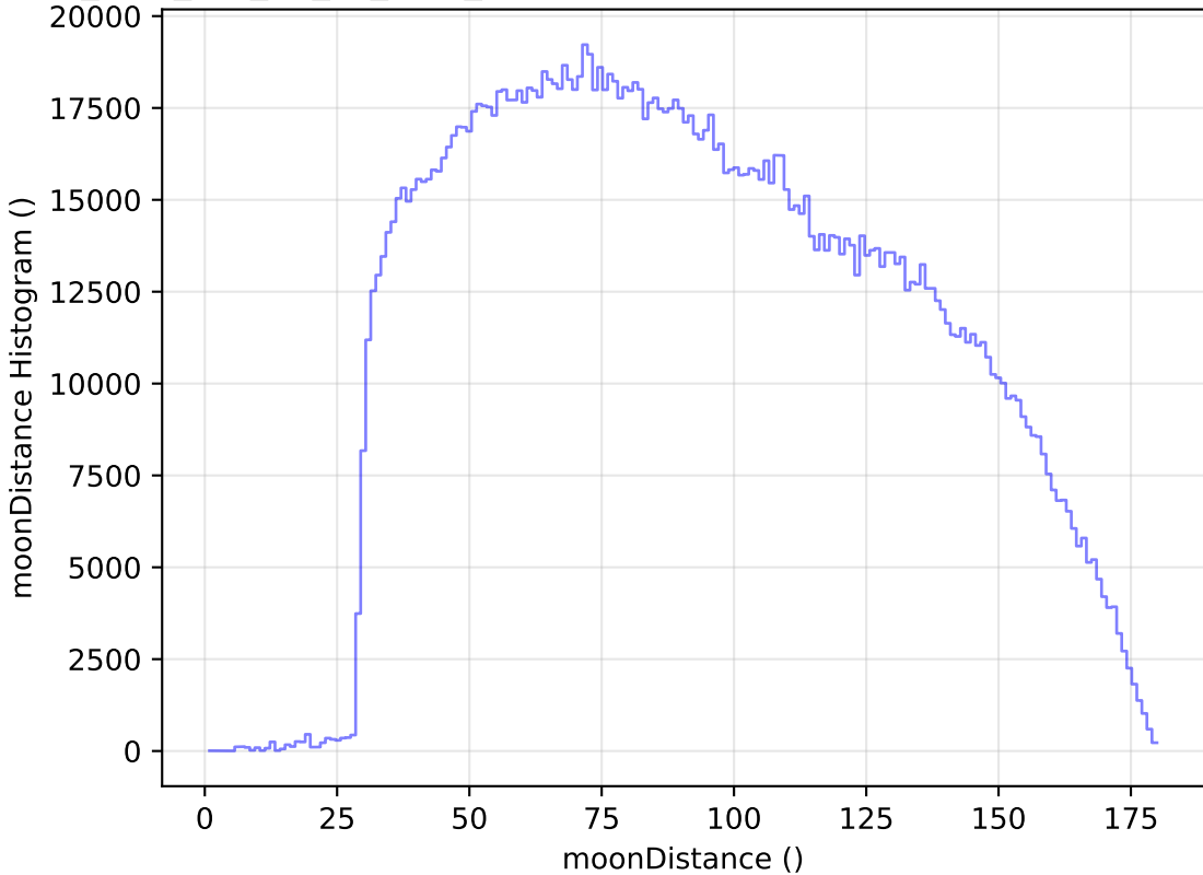
too_elab_r32_d2_gz_v3.4_10yrs All sky all bands: moonDistance Histogram
