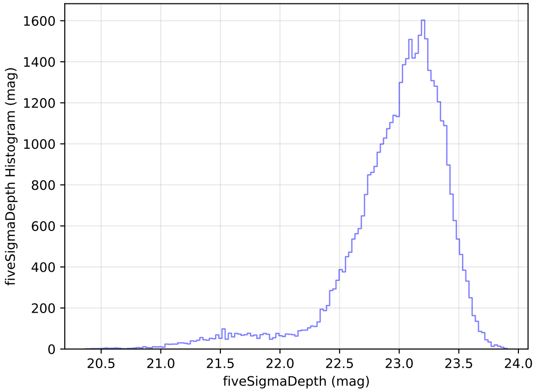
too_elab_r32_d2_gz_v3.4_10yrs Yr 1 z band: fiveSigmaDepth Histogram
