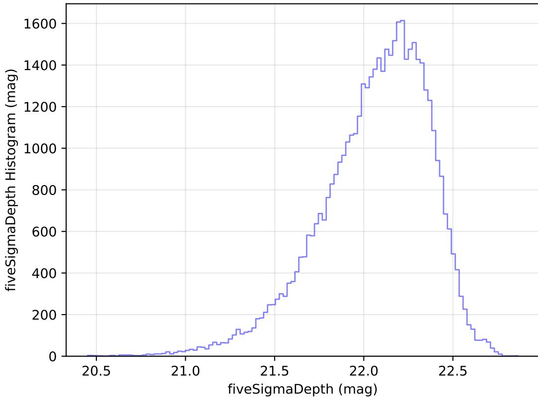
too_elab_r32_d2_gz_v3.4_10yrs Yr 1 y band: fiveSigmaDepth Histogram
