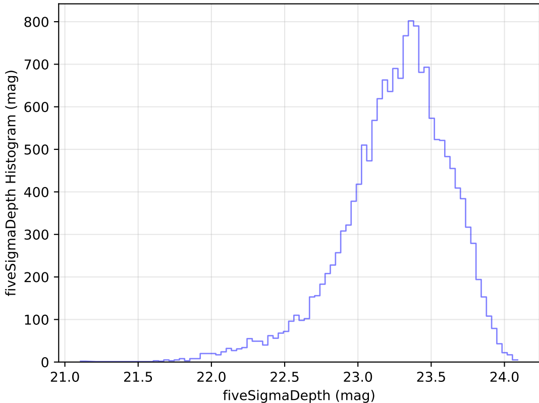
too_elab_r32_d2_gz_v3.4_10yrs Yr 1 u band: fiveSigmaDepth Histogram
