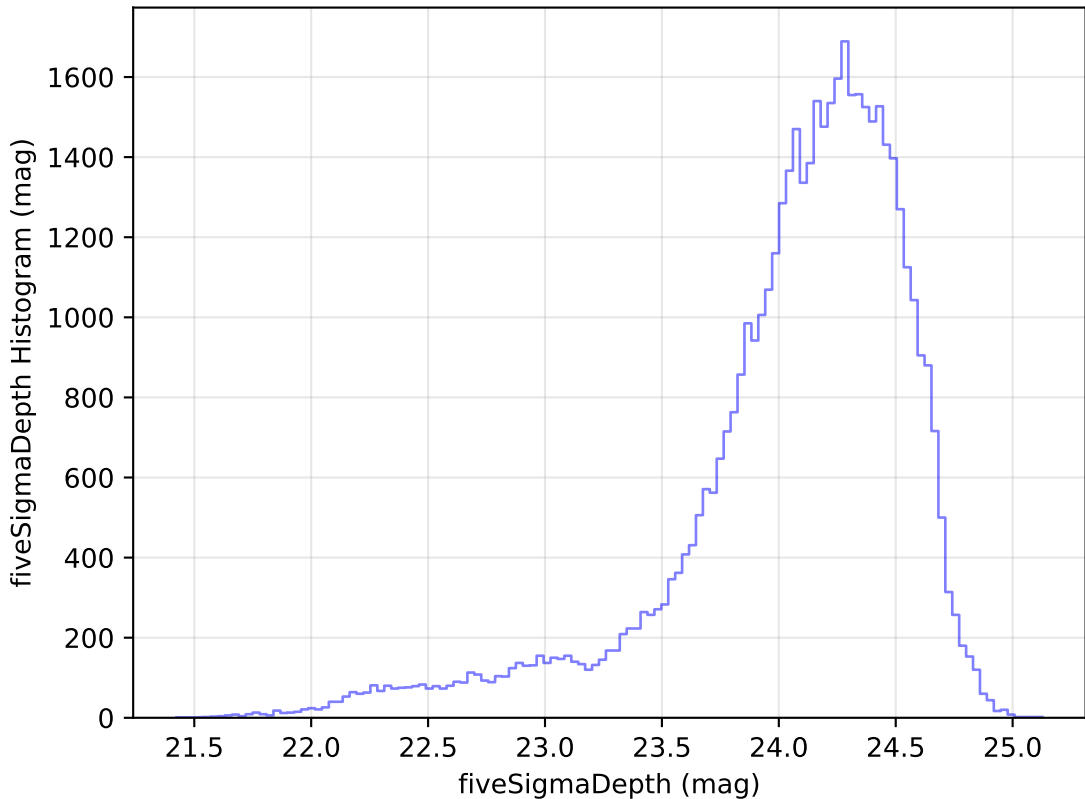
too_elab_r32_d2_gz_v3.4_10yrs Yr 1 r band: fiveSigmaDepth Histogram
