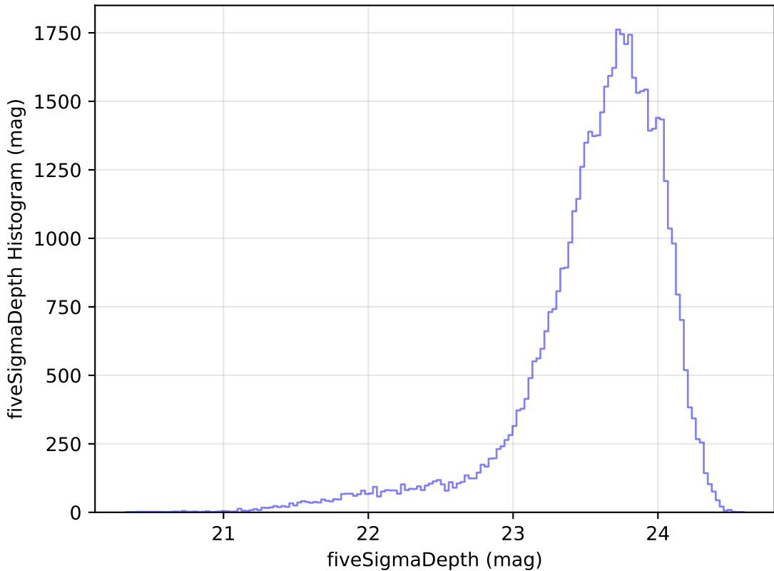
too_elab_r32_d2_gz_v3.4_10yrs Yr 1 i band: fiveSigmaDepth Histogram
