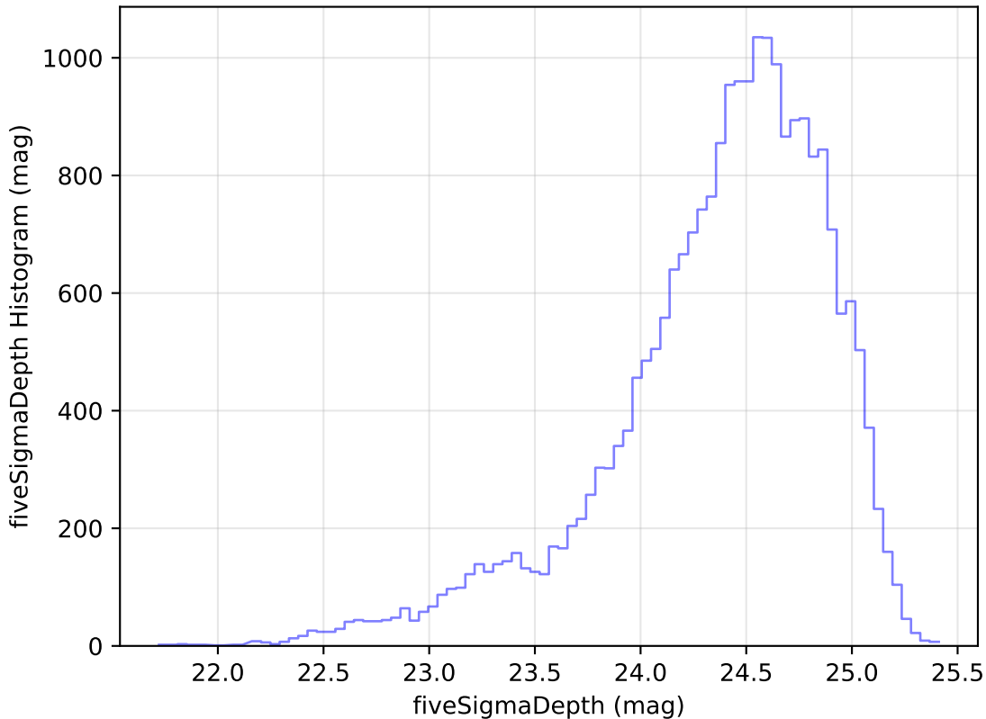
too_elab_r32_d2_gz_v3.4_10yrs Yr 1 g band: fiveSigmaDepth Histogram
