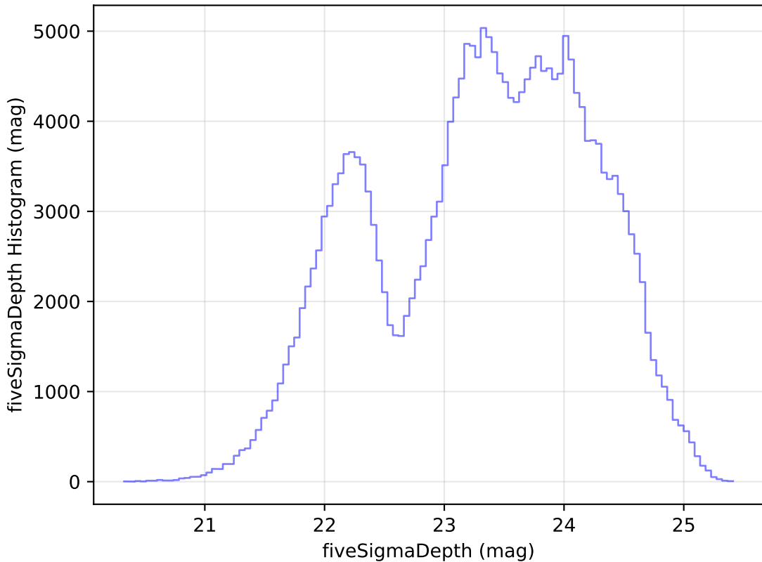
too_elab_r32_d2_gz_v3.4_10yrs Yr 1 all bands: fiveSigmaDepth Histogram
