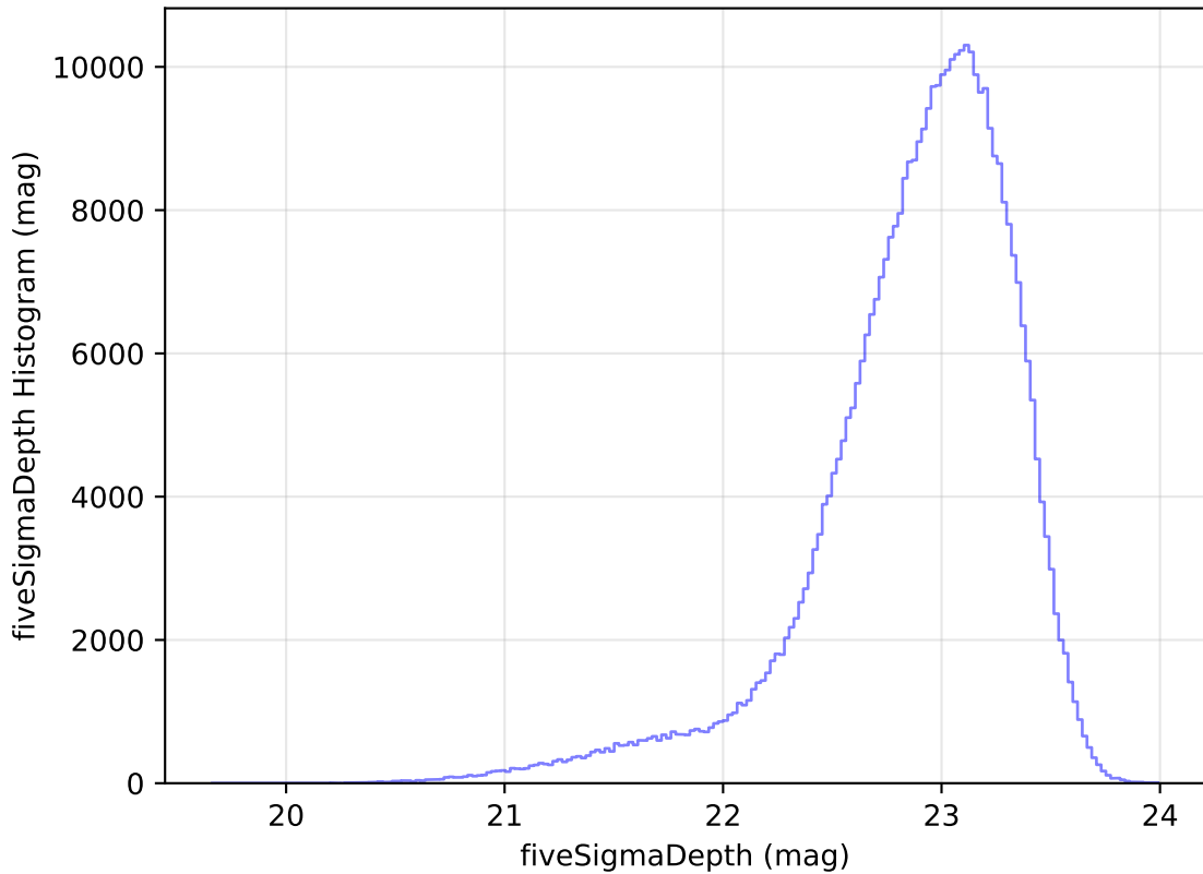
too_elab_r32_d2_gz_v3.4_10yrs WFD z band: fiveSigmaDepth Histogram
