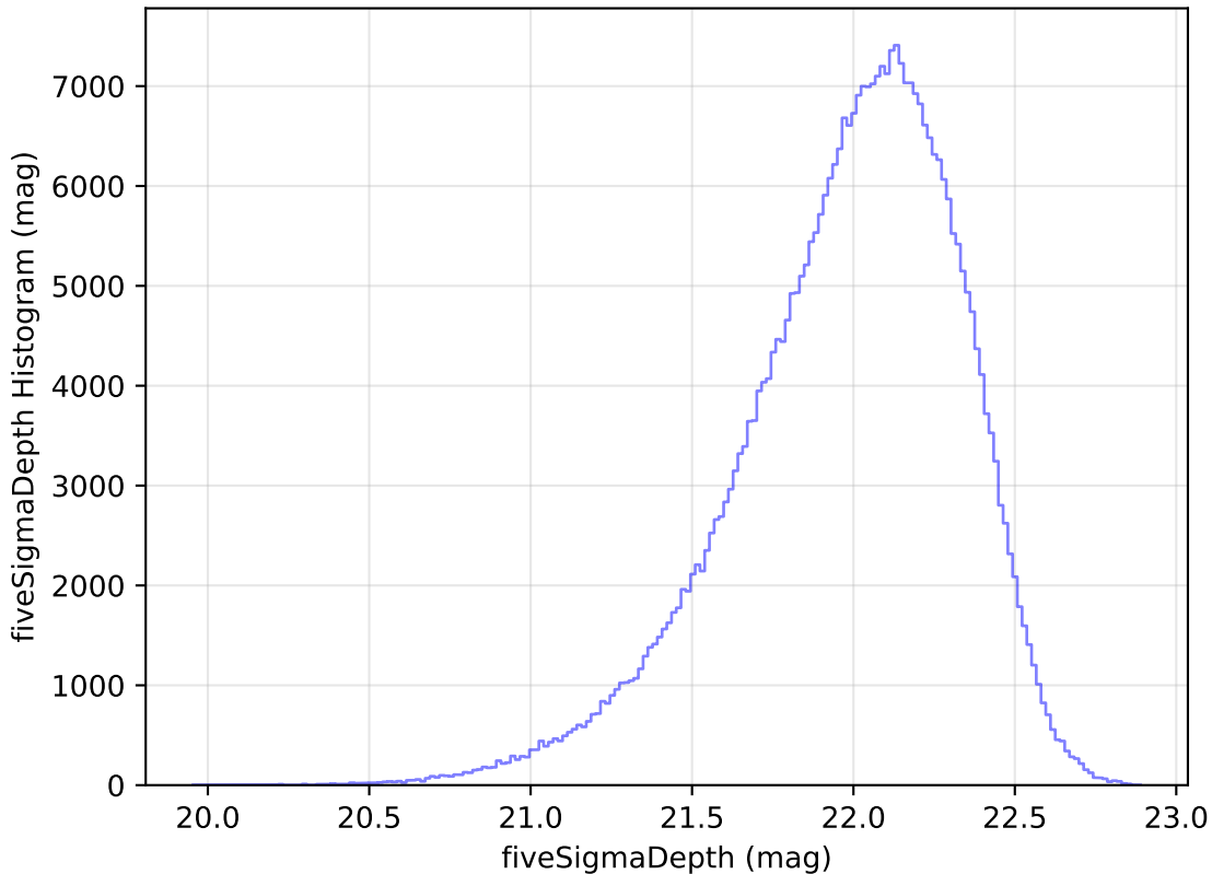
too_elab_r32_d2_gz_v3.4_10yrs WFD y band: fiveSigmaDepth Histogram
