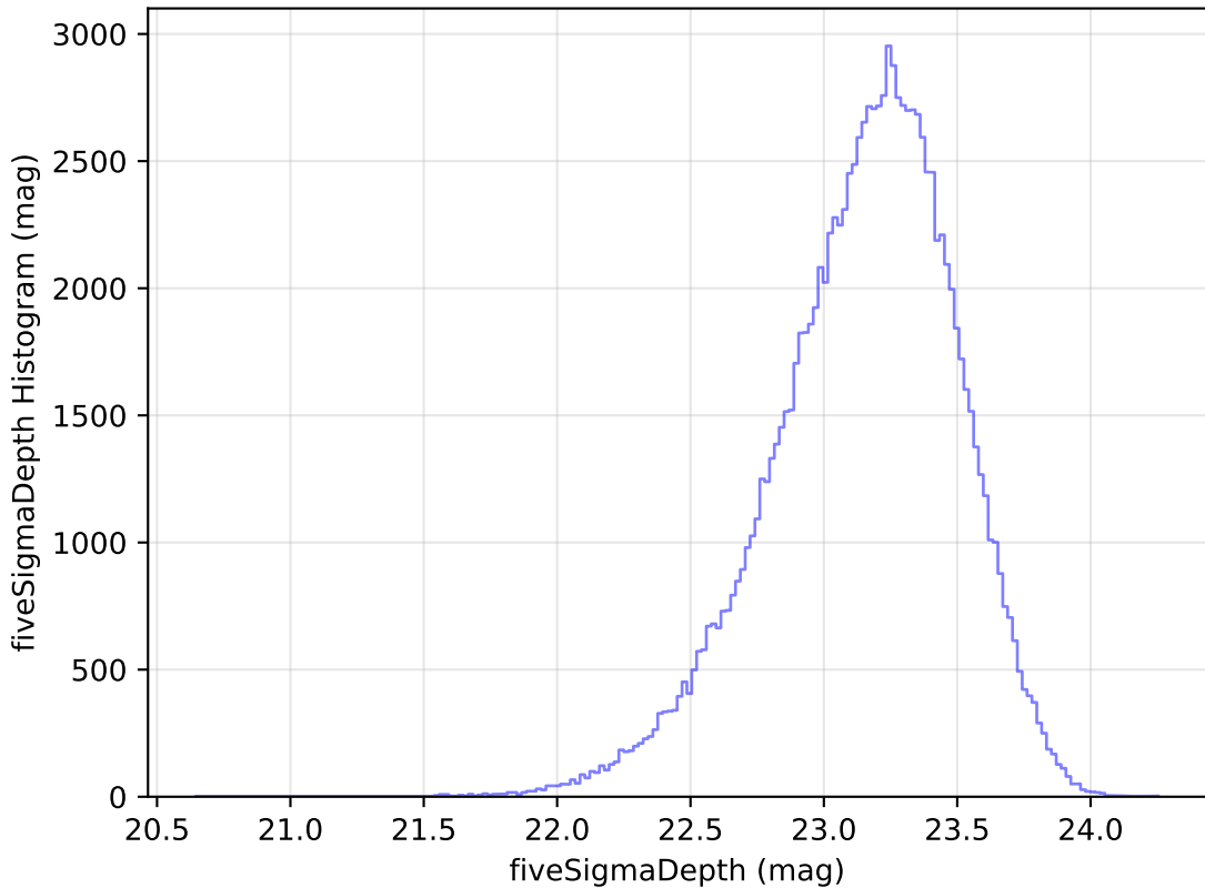
too_elab_r32_d2_gz_v3.4_10yrs WFD u band: fiveSigmaDepth Histogram
