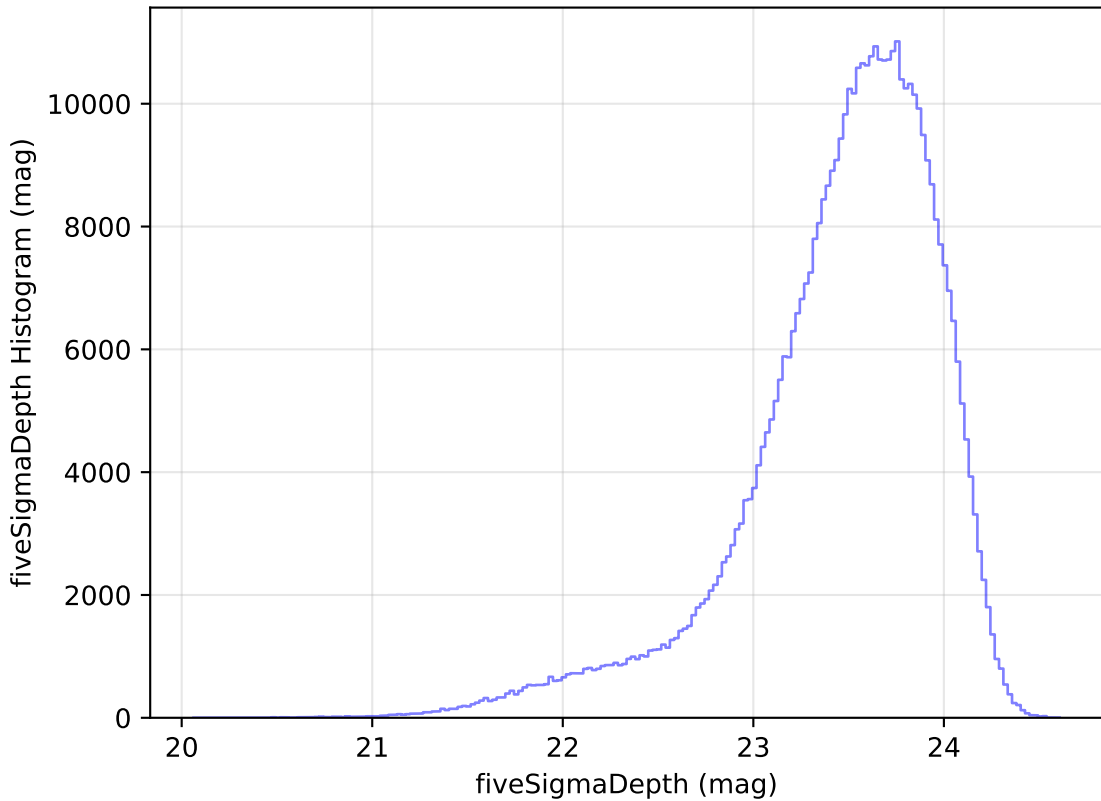
too_elab_r32_d2_gz_v3.4_10yrs WFD i band: fiveSigmaDepth Histogram
