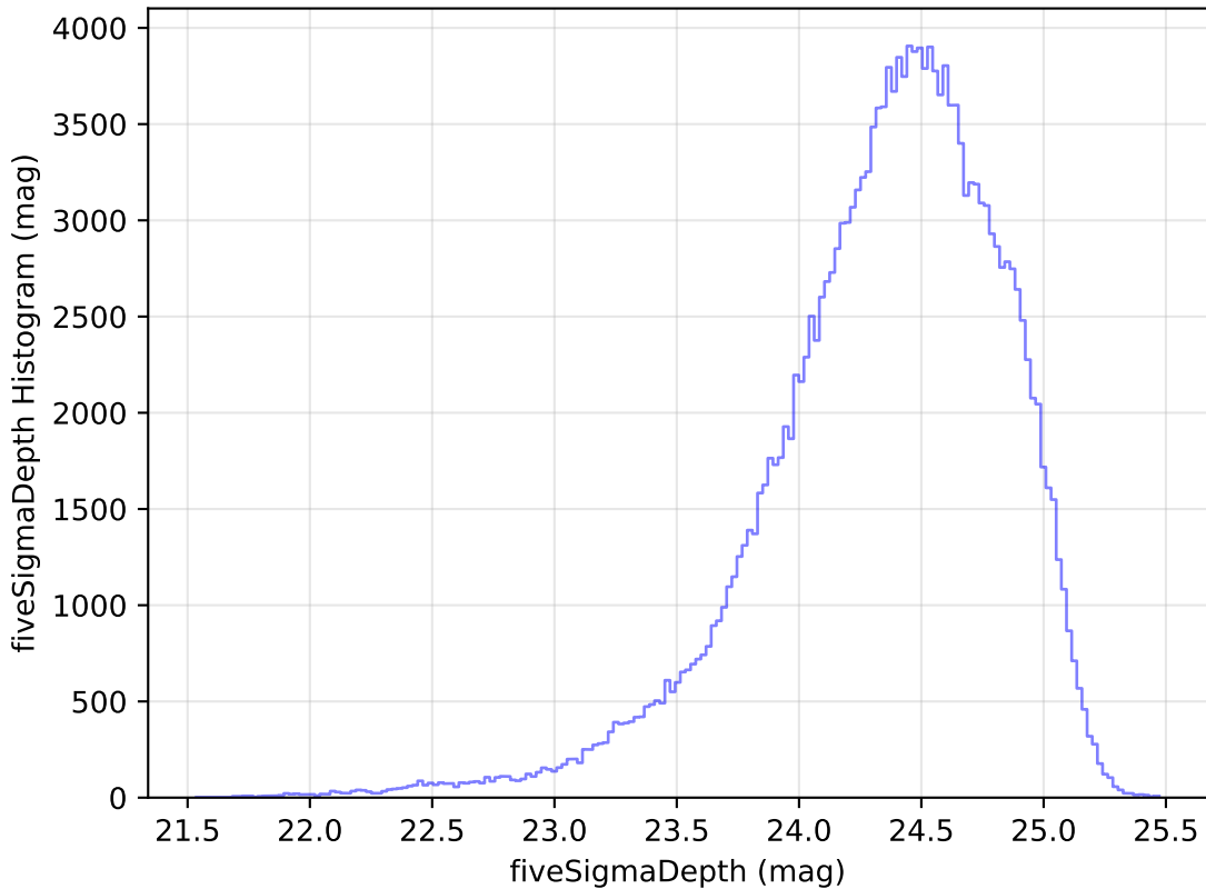
too_elab_r32_d2_gz_v3.4_10yrs WFD g band: fiveSigmaDepth Histogram
