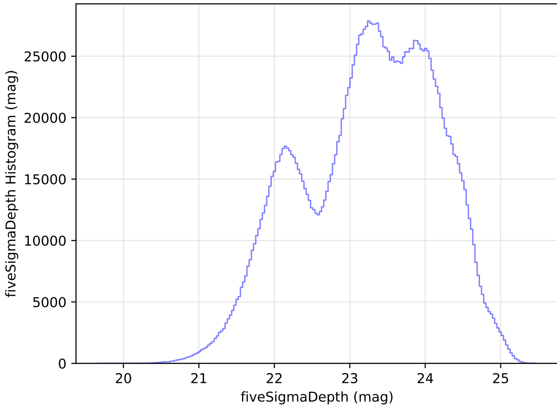
too_elab_r32_d2_gz_v3.4_10yrs WFD all bands: fiveSigmaDepth Histogram
