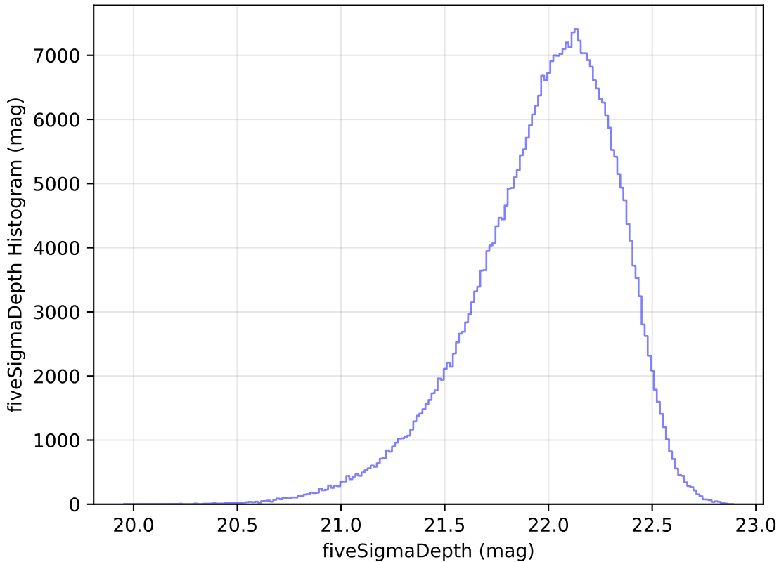
too_elab_r32_d2_gz_v3.4_10yrs All sky y band: fiveSigmaDepth Histogram
