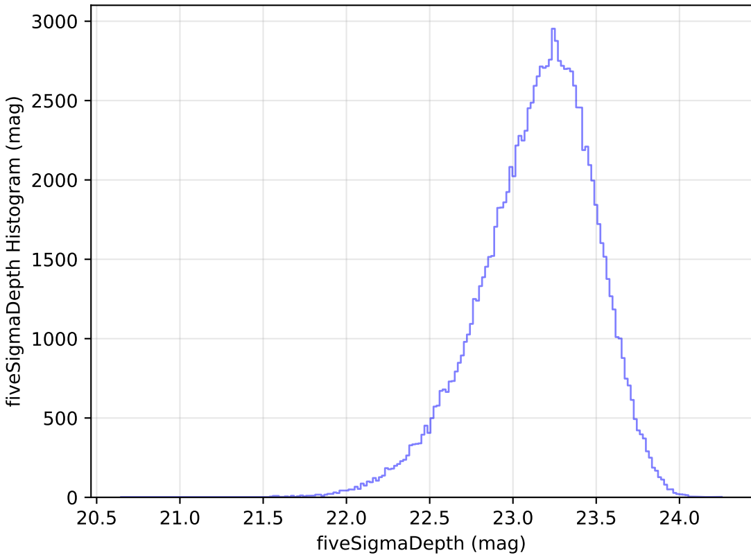
too_elab_r32_d2_gz_v3.4_10yrs All sky u band: fiveSigmaDepth Histogram
