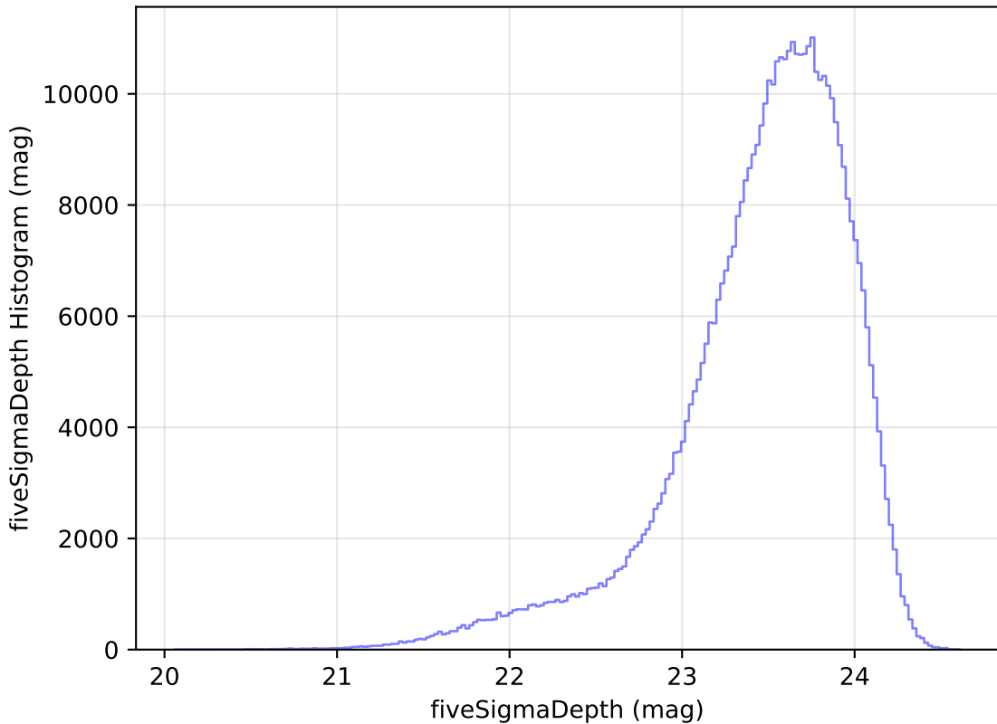
too_elab_r32_d2_gz_v3.4_10yrs All sky i band: fiveSigmaDepth Histogram
