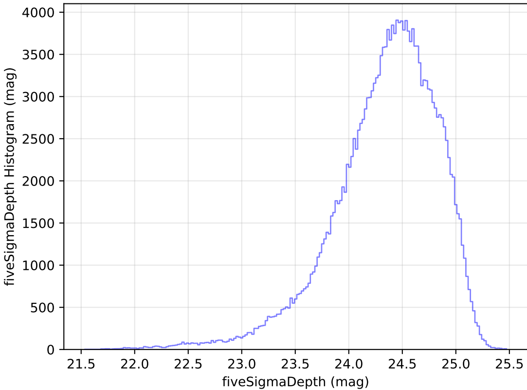
too_elab_r32_d2_gz_v3.4_10yrs All sky g band: fiveSigmaDepth Histogram
