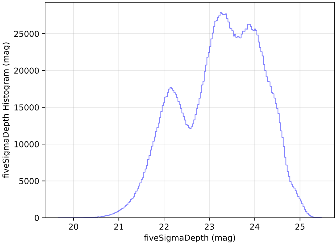
too_elab_r32_d2_gz_v3.4_10yrs All sky all bands: fiveSigmaDepth Histogram
