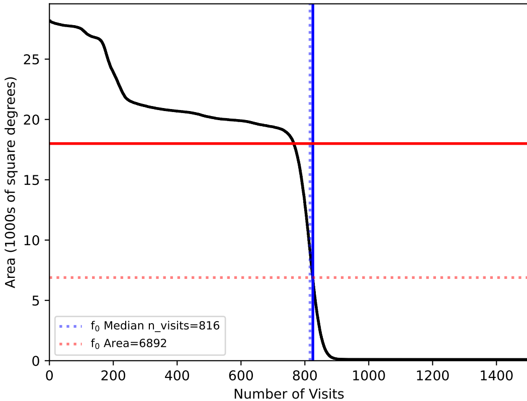
too_elab_r32_d2_gz_v3.4_10yrs All sky: fO
