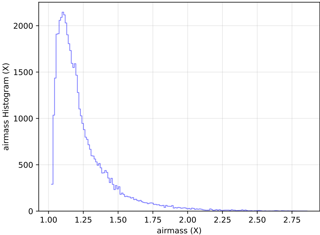
too_elab_r32_d2_gz_v3.4_10yrs Yr 1 y band: airmass Histogram
