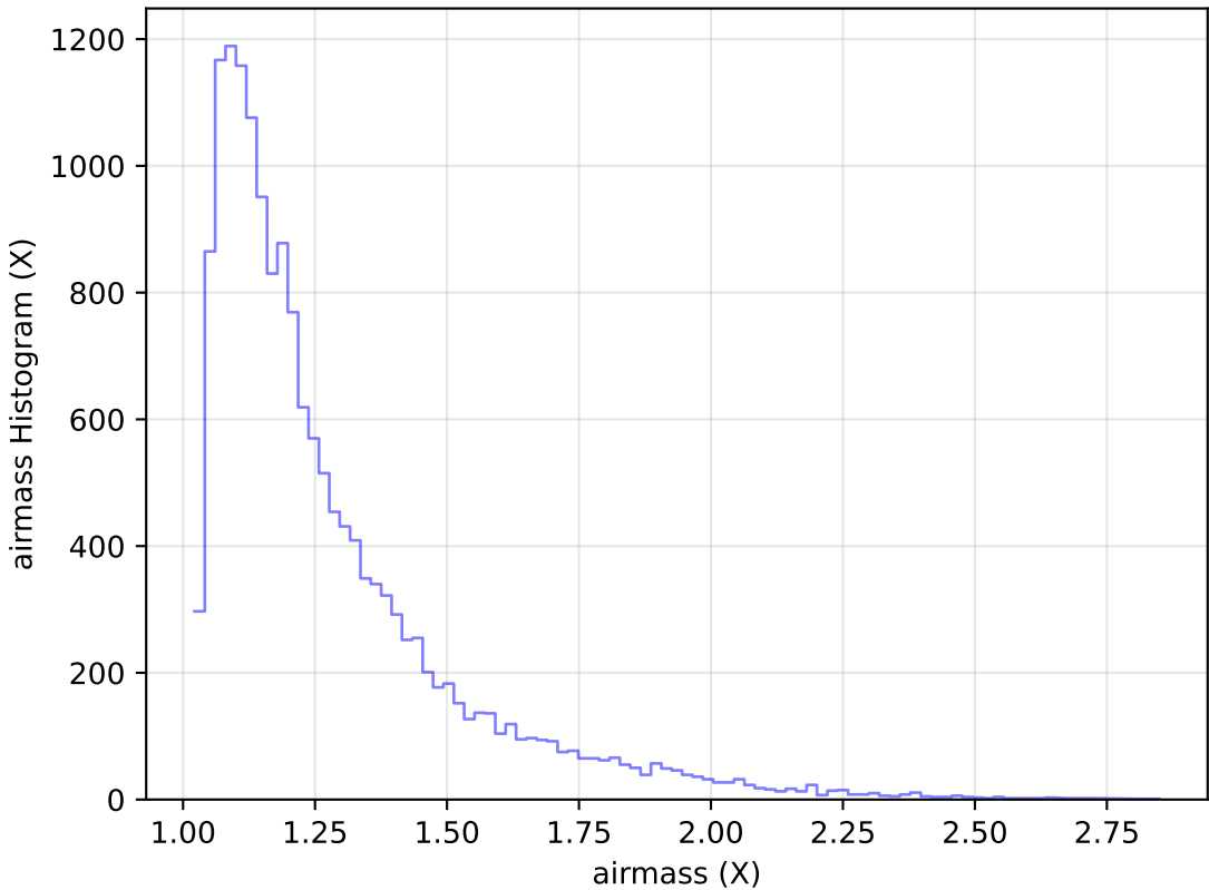
too_elab_r32_d2_gz_v3.4_10yrs Yr 1 u band: airmass Histogram
