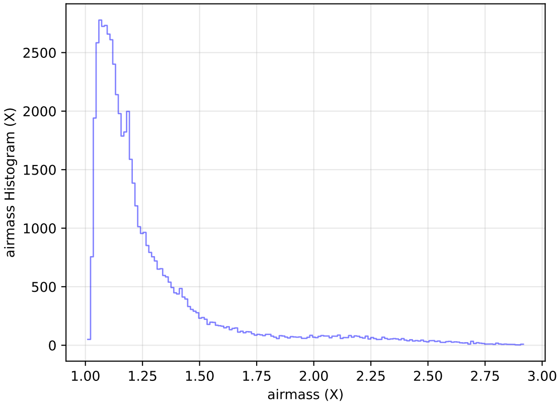
too_elab_r32_d2_gz_v3.4_10yrs Yr 1 i band: airmass Histogram
