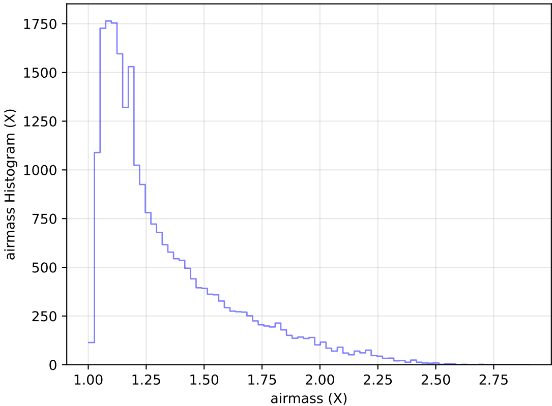
too_elab_r32_d2_gz_v3.4_10yrs Yr 1 g band: airmass Histogram
