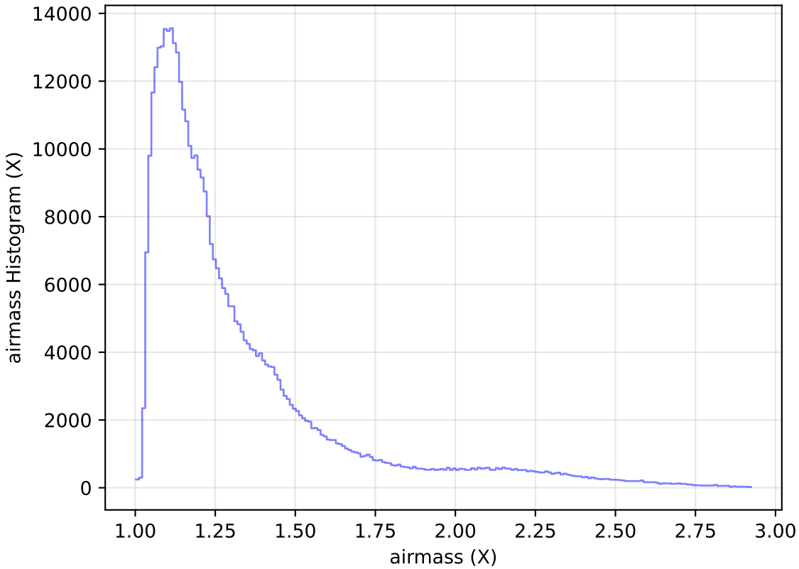
too_elab_r32_d2_gz_v3.4_10yrs WFD z band: airmass Histogram
