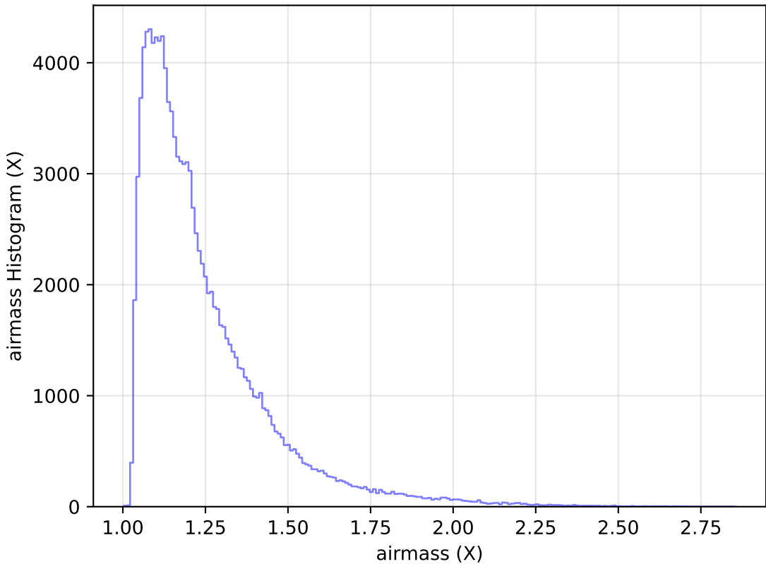
too_elab_r32_d2_gz_v3.4_10yrs WFD u band: airmass Histogram
