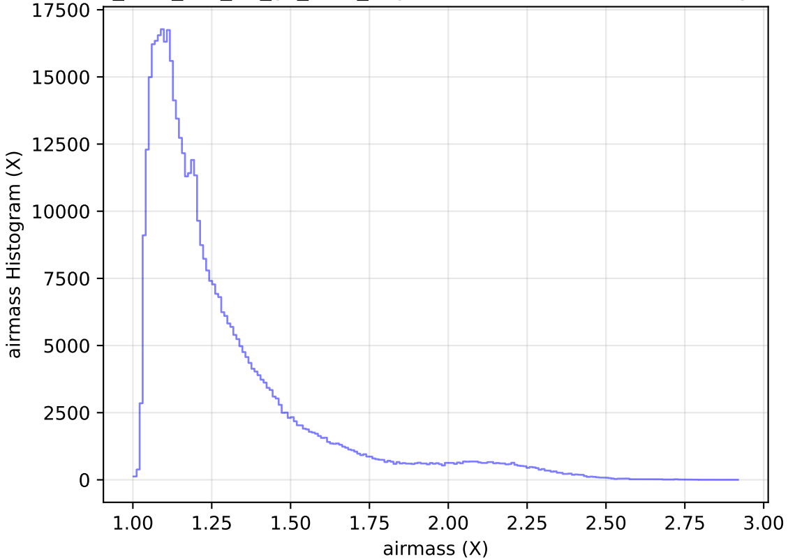
too_elab_r32_d2_gz_v3.4_10yrs WFD r band: airmass Histogram
