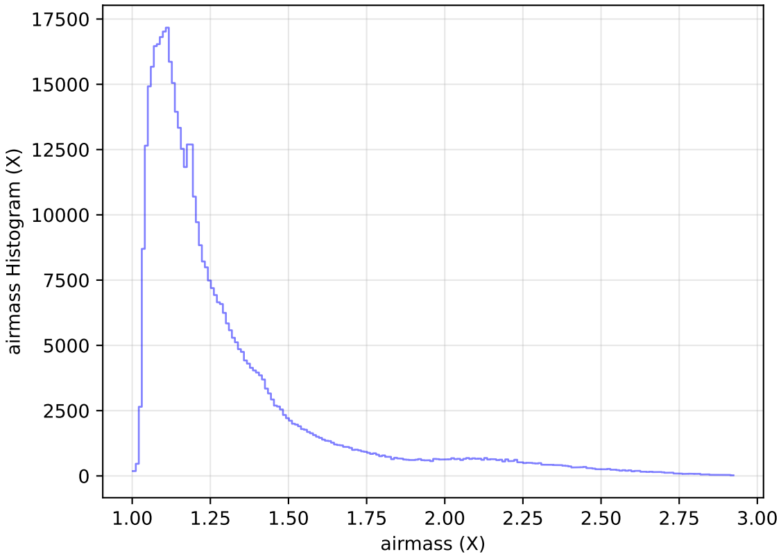
too_elab_r32_d2_gz_v3.4_10yrs WFD i band: airmass Histogram
