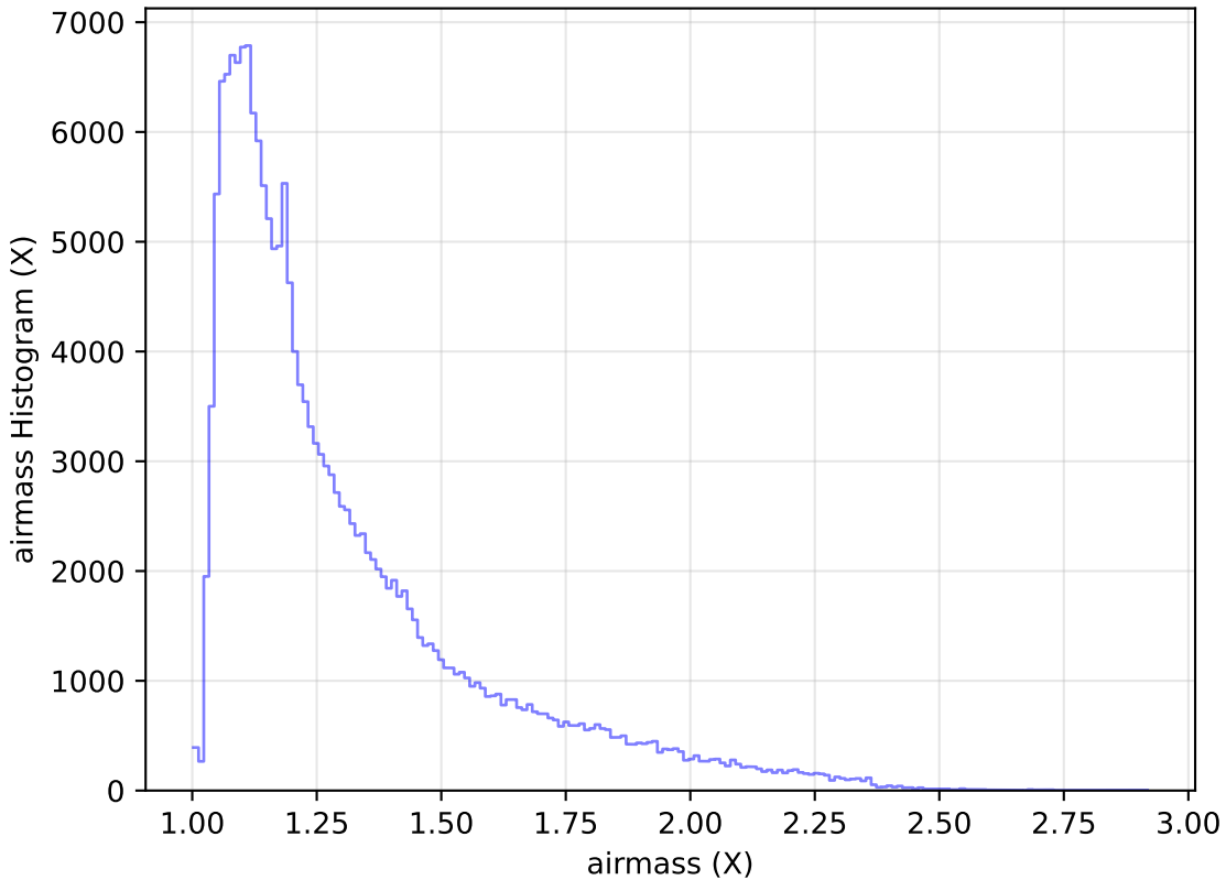
too_elab_r32_d2_gz_v3.4_10yrs WFD g band: airmass Histogram
