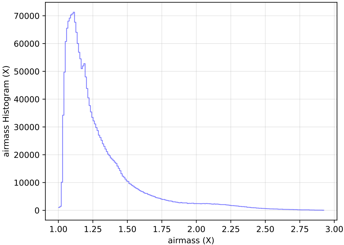
too_elab_r32_d2_gz_v3.4_10yrs WFD all bands: airmass Histogram
