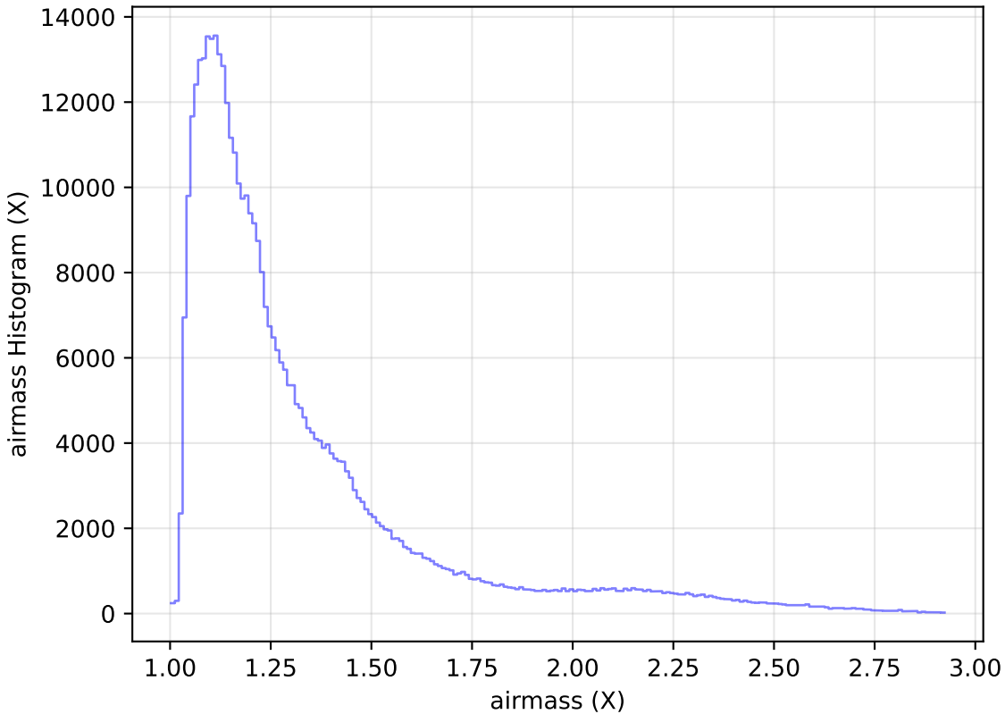
too_elab_r32_d2_gz_v3.4_10yrs All sky z band: airmass Histogram
