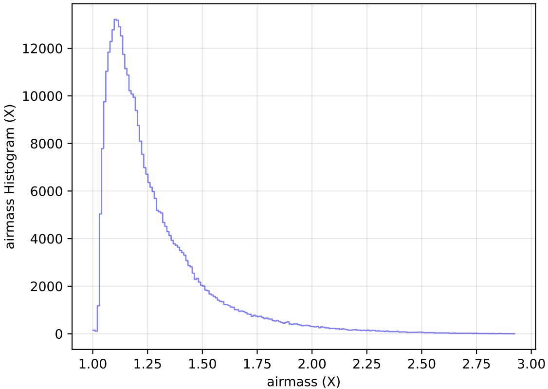
too_elab_r32_d2_gz_v3.4_10yrs All sky y band: airmass Histogram
