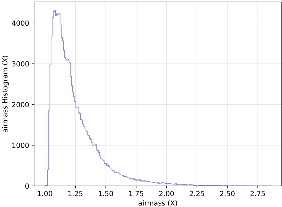
too_elab_r32_d2_gz_v3.4_10yrs All sky u band: airmass Histogram
