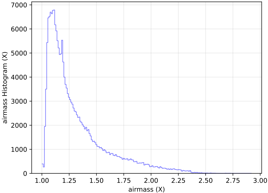
too_elab_r32_d2_gz_v3.4_10yrs All sky g band: airmass Histogram
