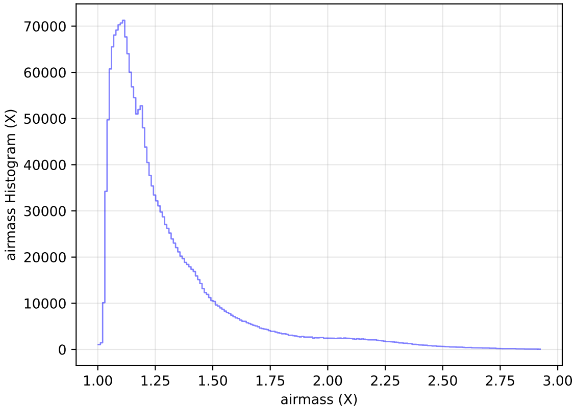
too_elab_r32_d2_gz_v3.4_10yrs All sky all bands: airmass Histogram
