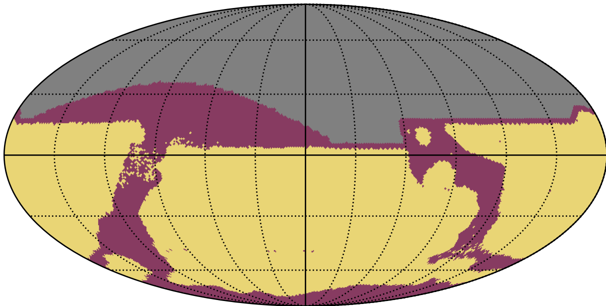
too_elab_r32_d2_gz_v3.4_10yrs All sky: RapidRevisits
