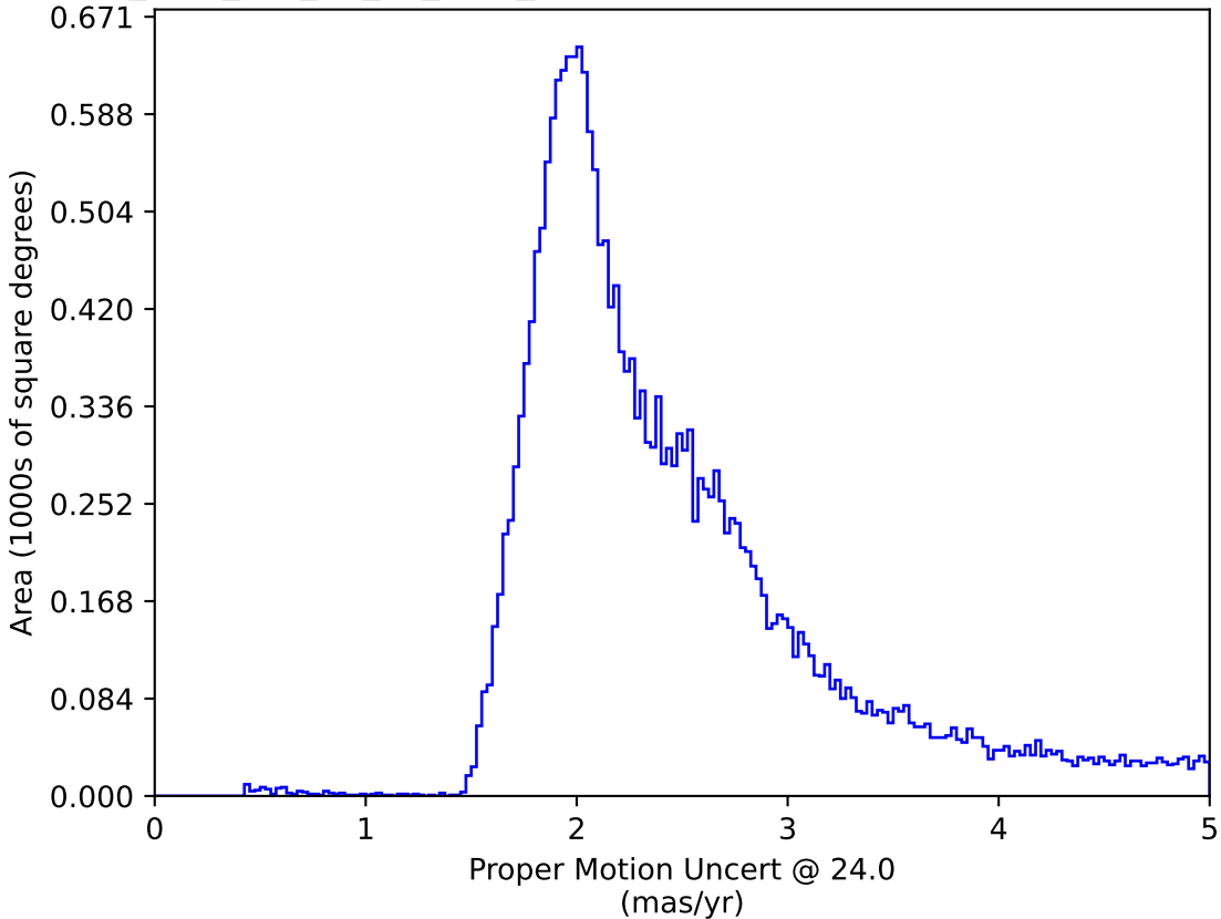
too_elab_r32_d2_gz_v3.4_10yrs All sky: Proper Motion Uncert @ 24.0
