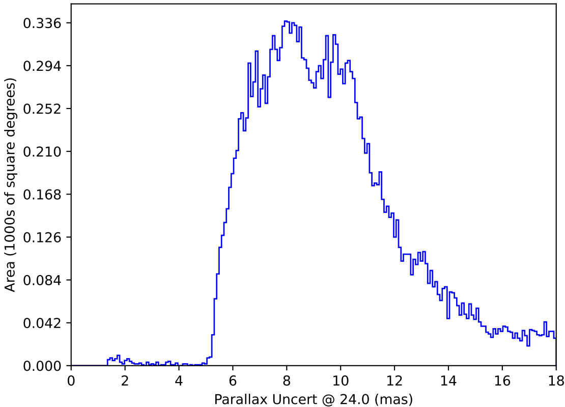
too_elab_r32_d2_gz_v3.4_10yrs All sky: Parallax Uncert @ 24.0
