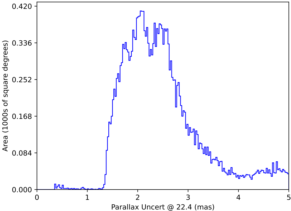
too_elab_r32_d2_gz_v3.4_10yrs All sky: Parallax Uncert @ 22.4
