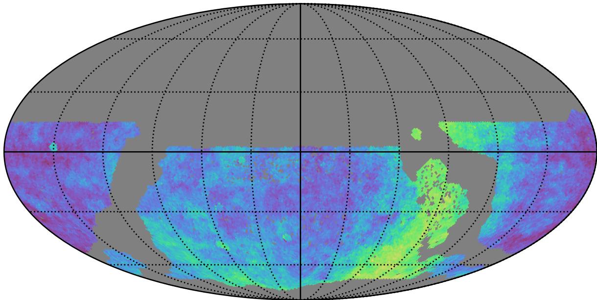
too_elab_r32_d2_gz_v3.4_10yrs WFD: Parallax Coverage @ 24.0
