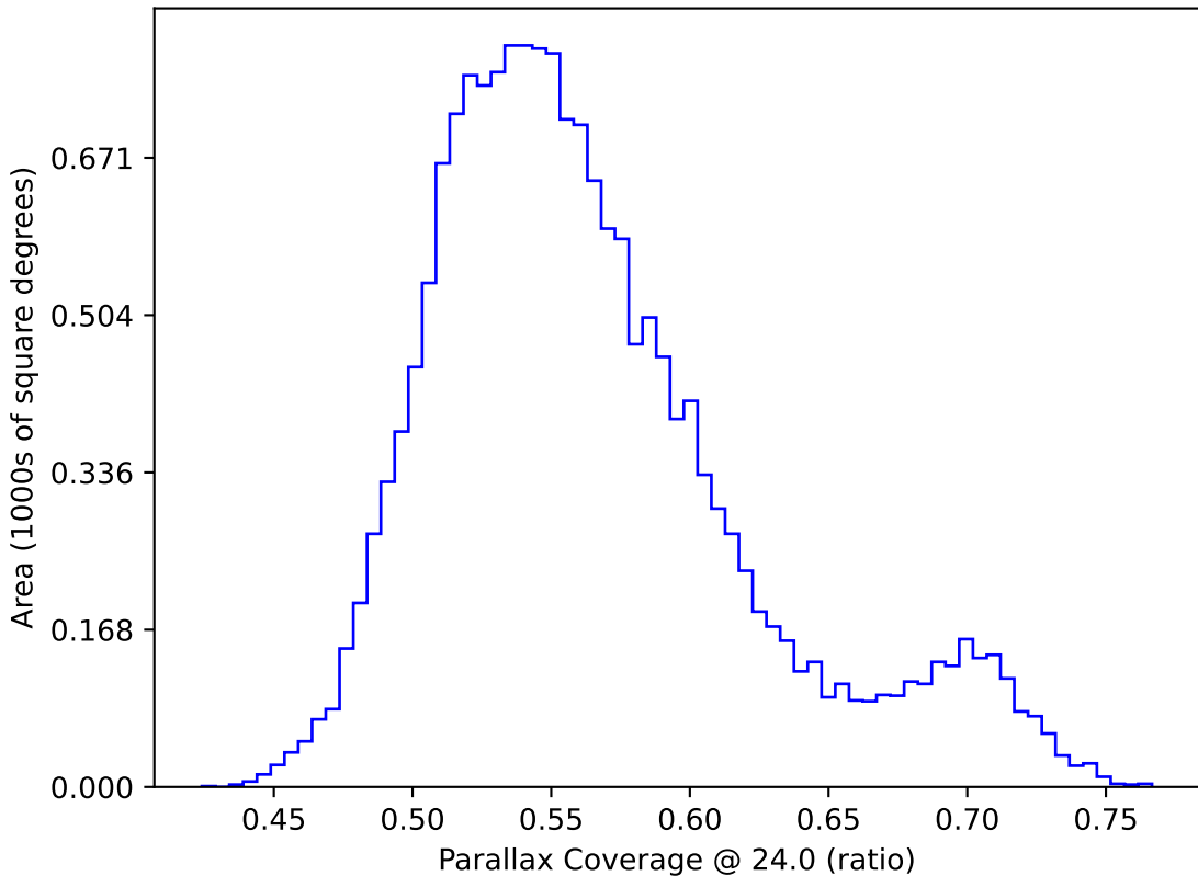
too_elab_r32_d2_gz_v3.4_10yrs WFD: Parallax Coverage @ 24.0
