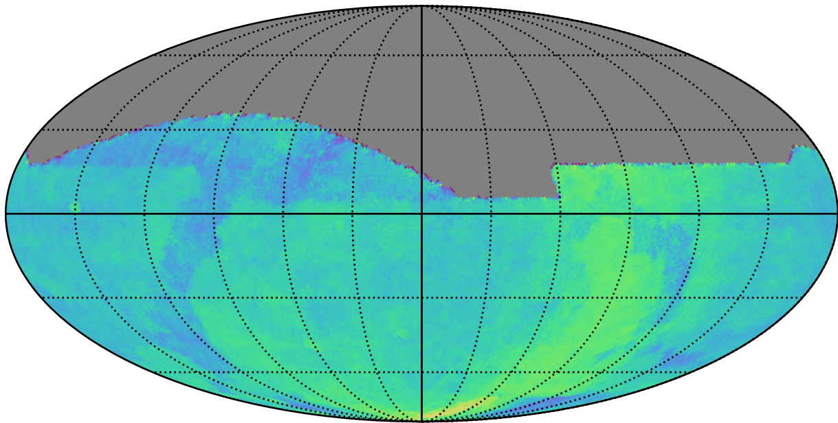
too_elab_r32_d2_gz_v3.4_10yrs All sky: Parallax Coverage @ 24.0
