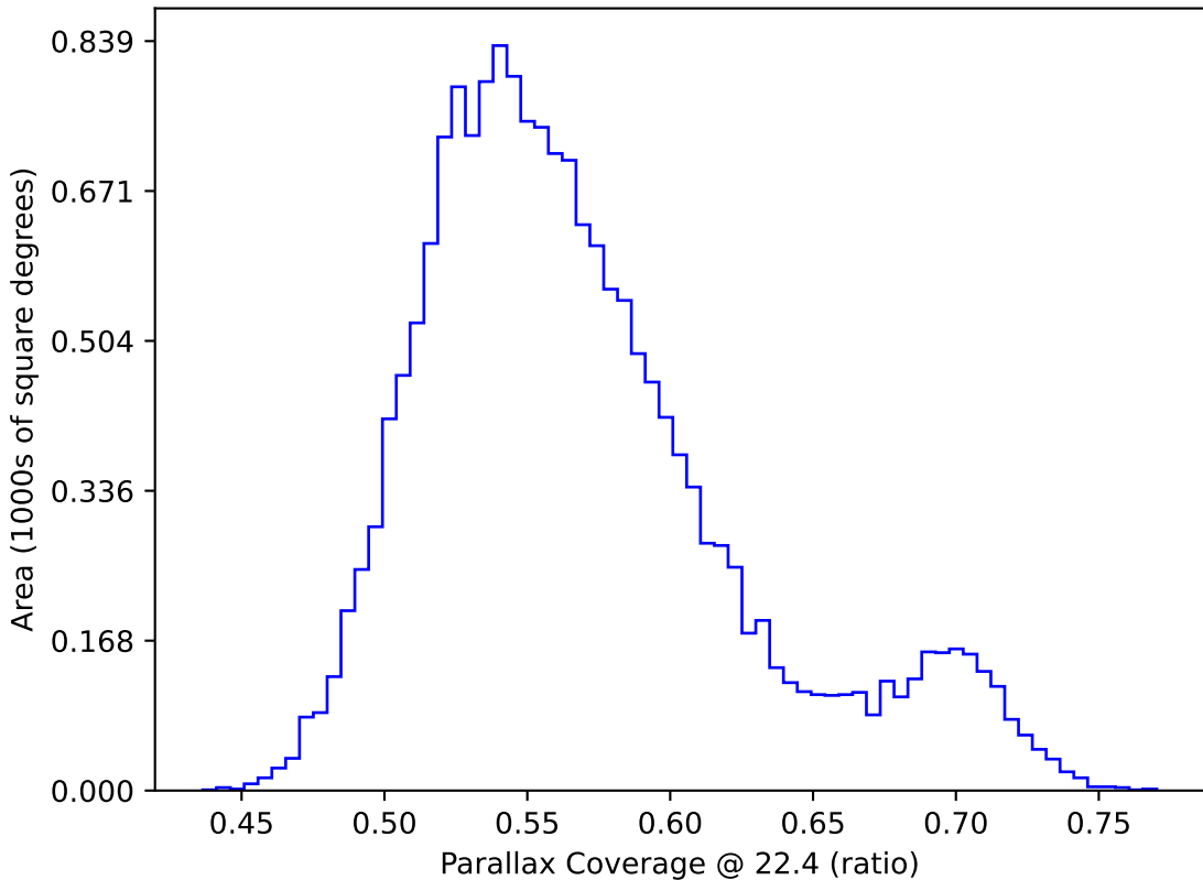
too_elab_r32_d2_gz_v3.4_10yrs WFD: Parallax Coverage @ 22.4
